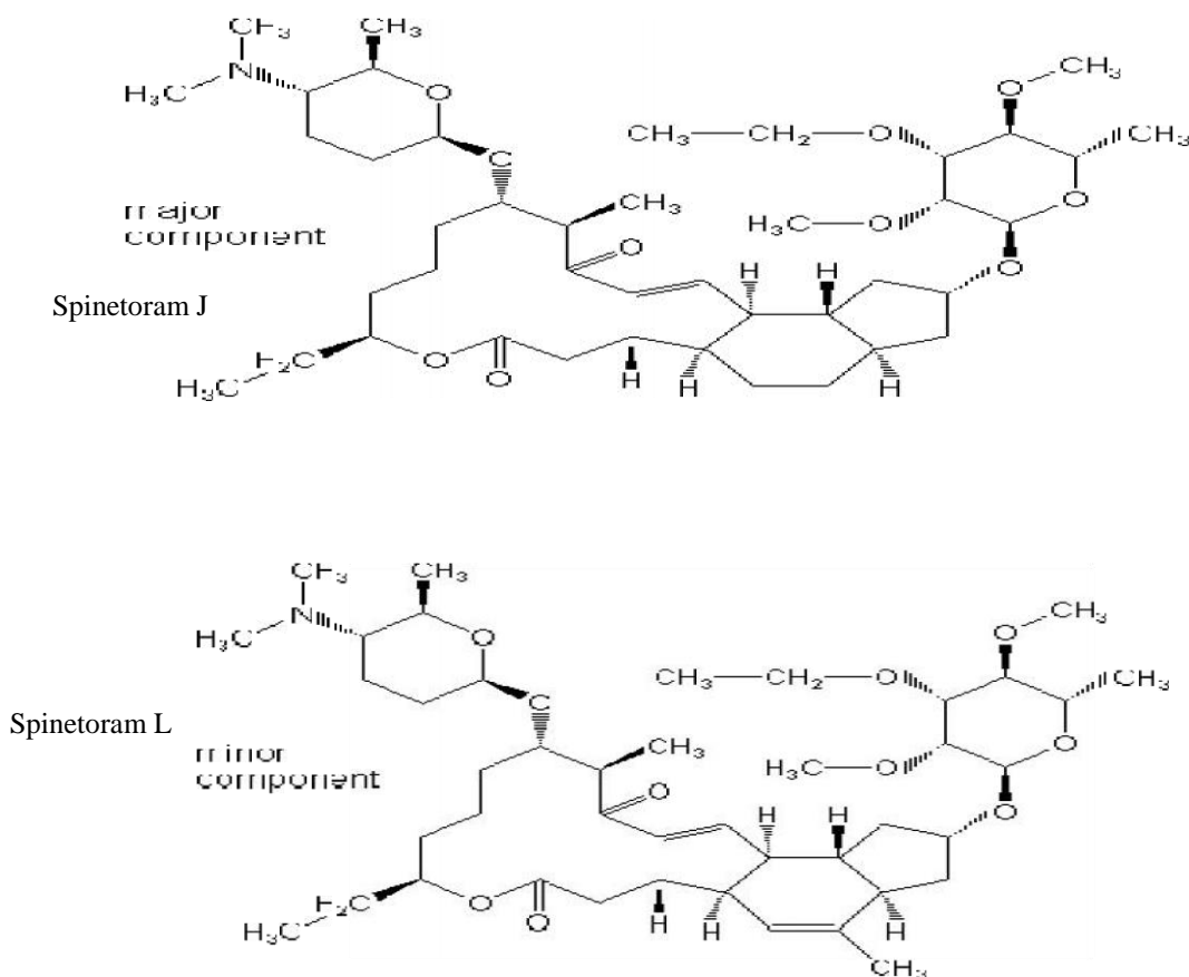
Fig. 1: Chemical structure of Spinetoram (J&L)
