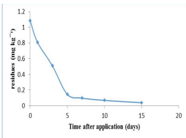
Fig. 2. Dissipation of spinetoram in/on tomato fruit with time.
